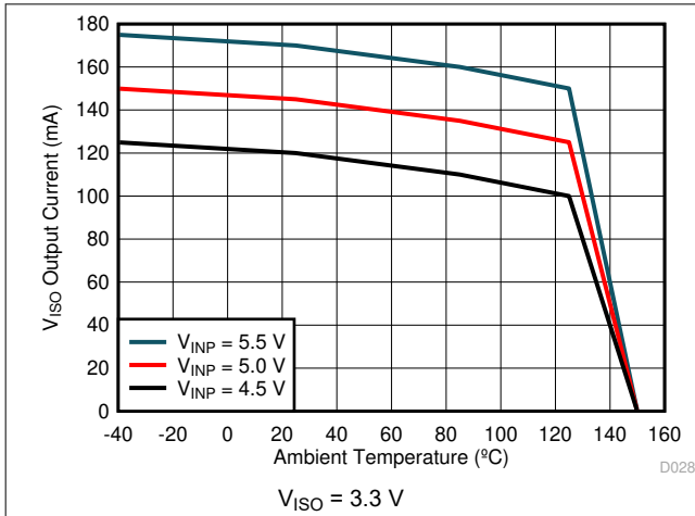
Figure 6-10. Maximum V_{ISO} Output Current vs. Temperature
