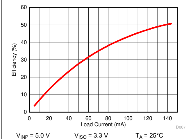
Figure 6-14. Power Supply Efficiency vs. Load Current ( I_{ISO} )
