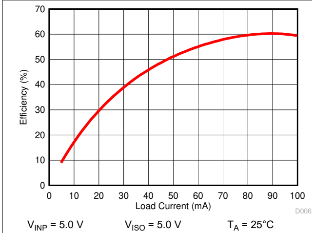
Figure 6-12. Power Supply Efficiency vs. Load Current ( I_{ISO} )
